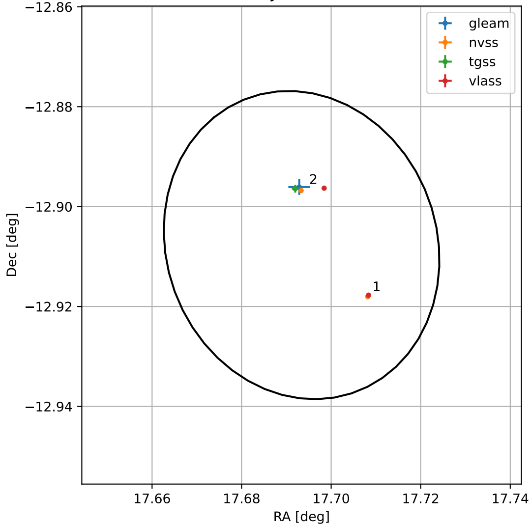
4FGL J0110.7-1254
