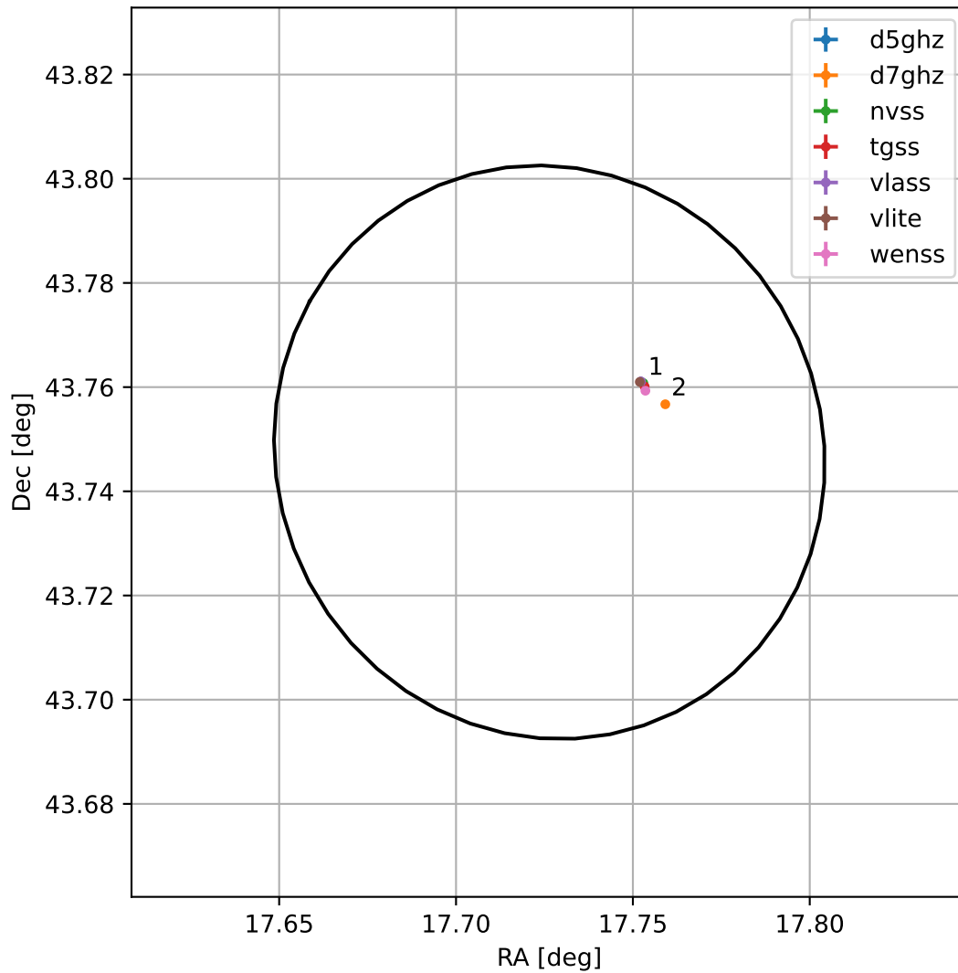
4FGL J0110.9+4344
