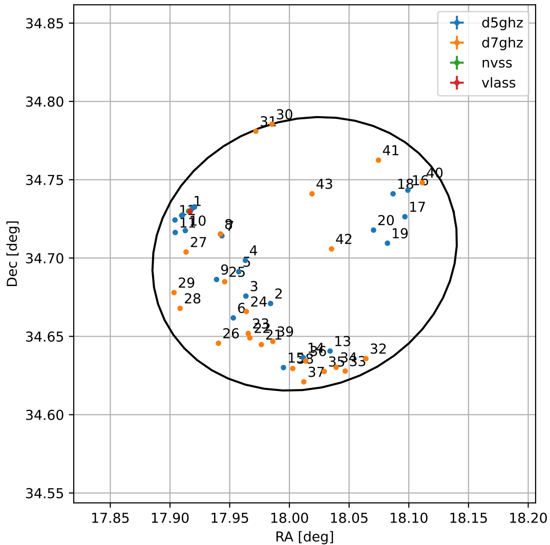
4FGL J0112.0+3442
