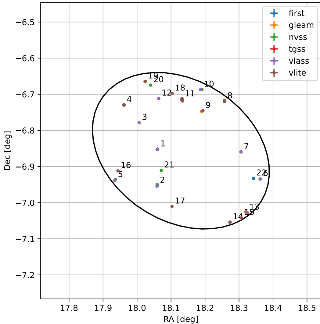
4FGL J0112.5-0651
