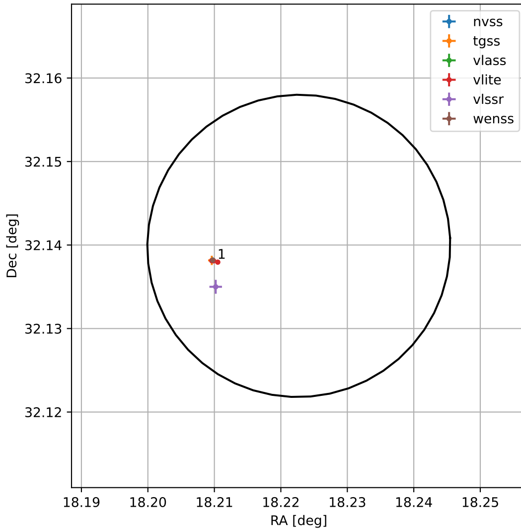
4FGL J0112.8+3208
