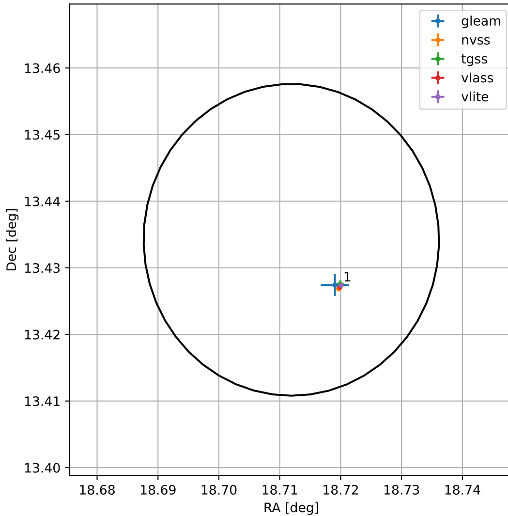
4FGL J0114.8+1326
