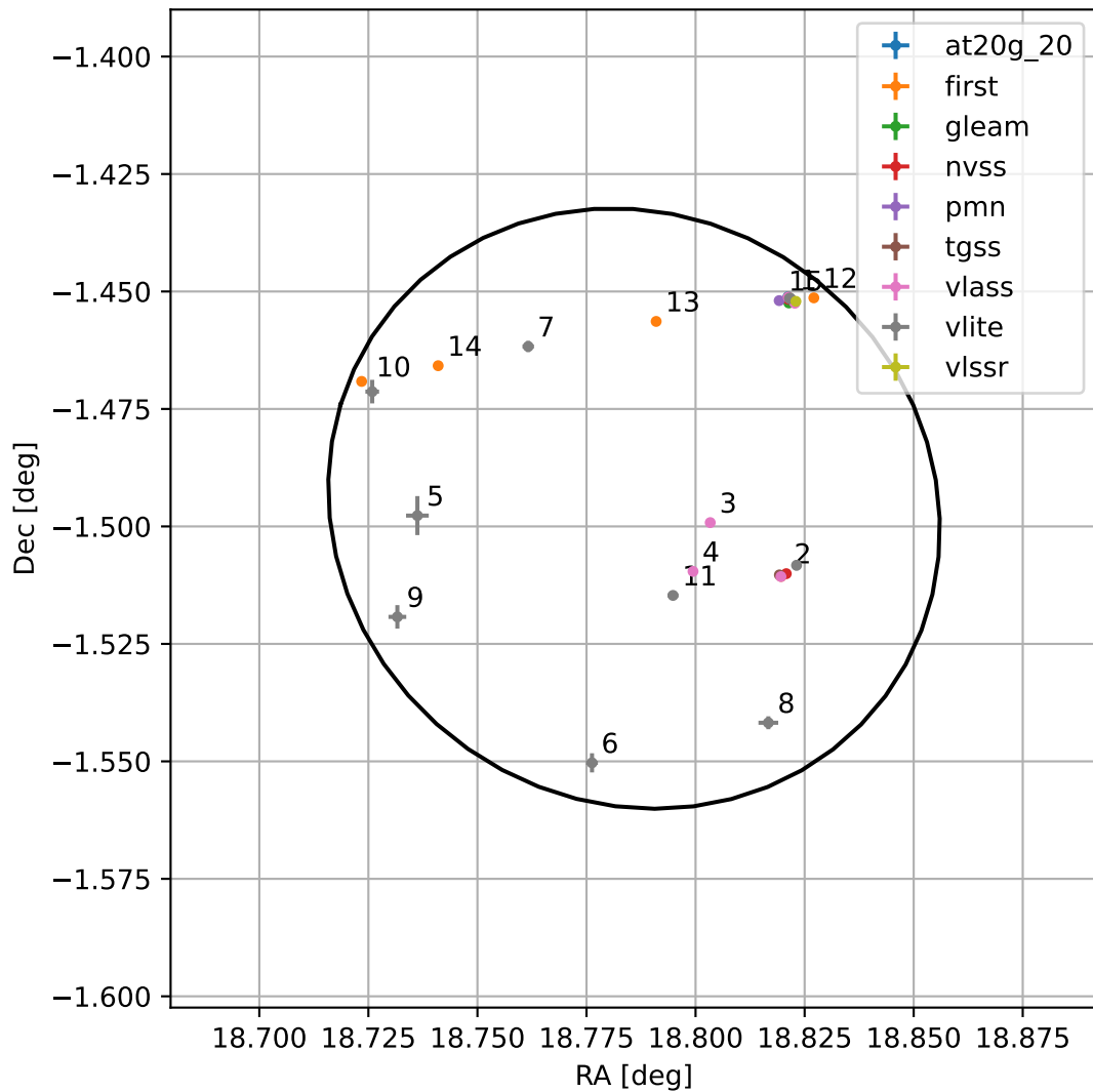
4FGL J0115.1-0129
