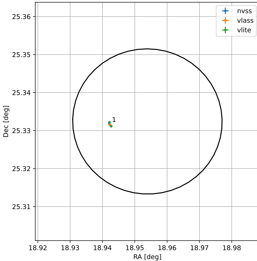
4FGL J0115.8+2519
