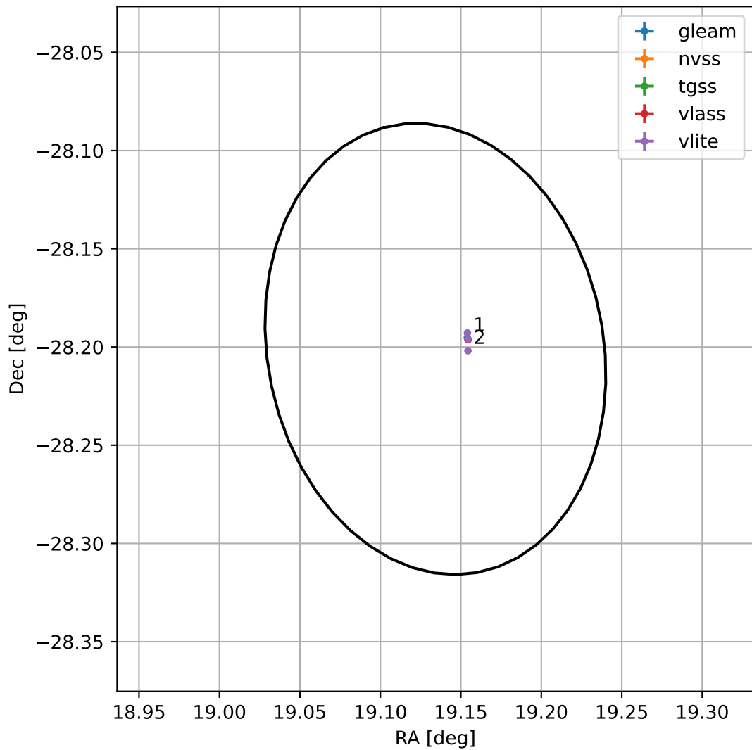
4FGL J0116.5-2812
