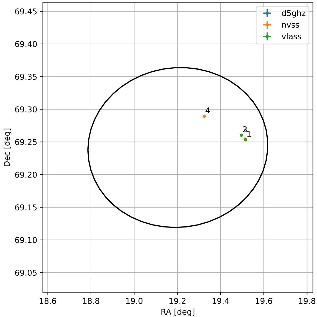
4FGL J0116.8+6914
