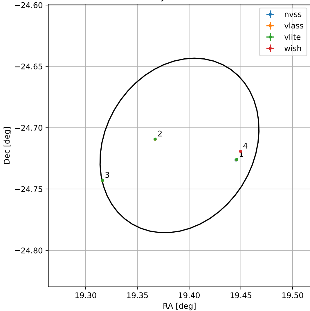
4FGL J0117.5-2442
