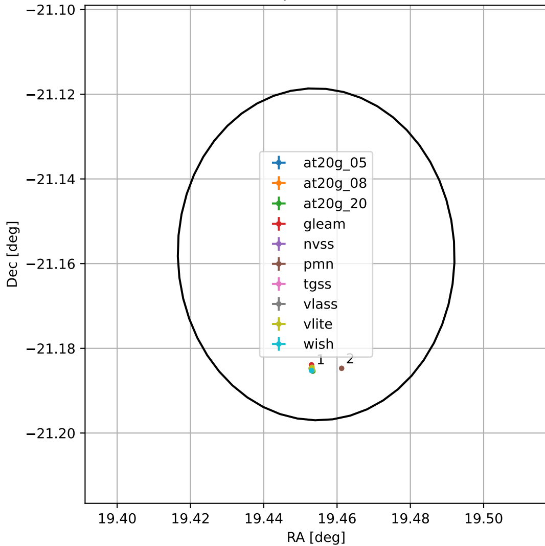
4FGL J0117.8-2109
