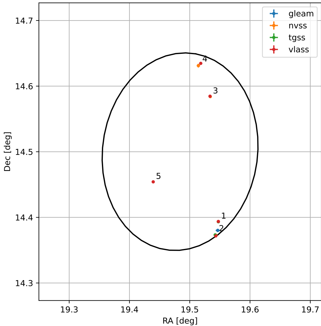
4FGL J0117.9+1430
