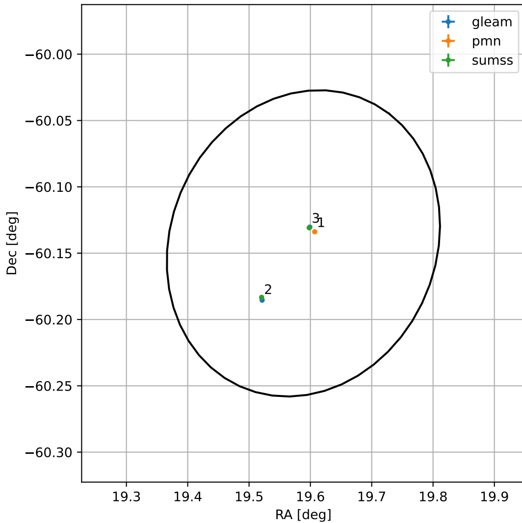
4FGL J0118.3-6008
