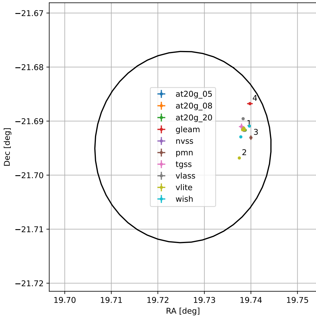
4FGL J0118.9-2141
