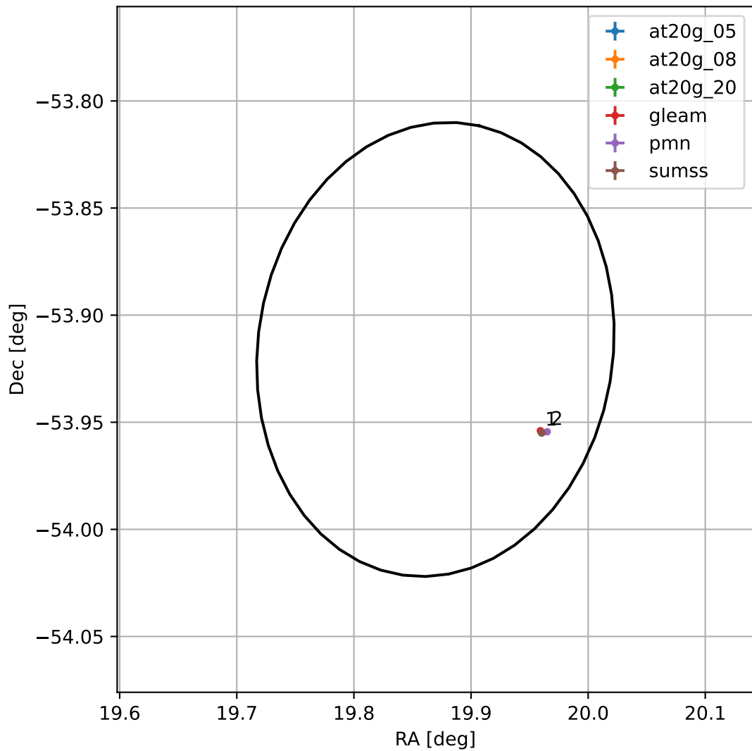
4FGL J0119.4-5354
