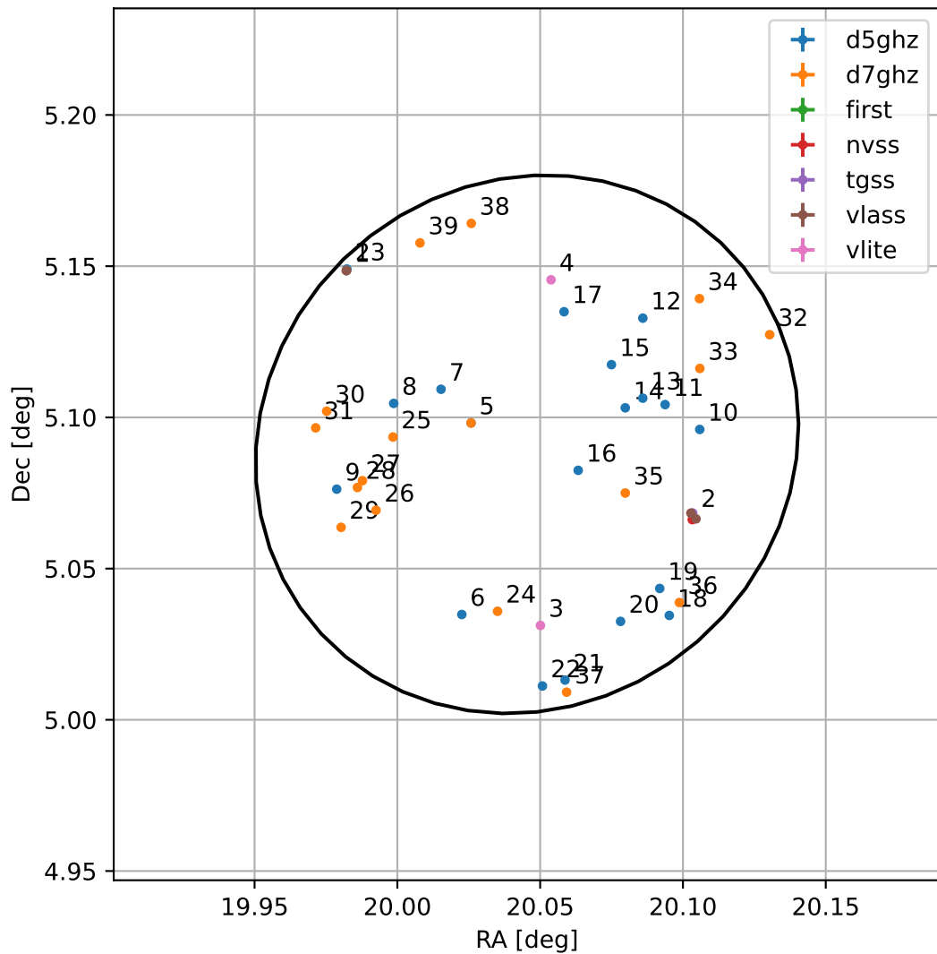
4FGL J0120.1+0505
