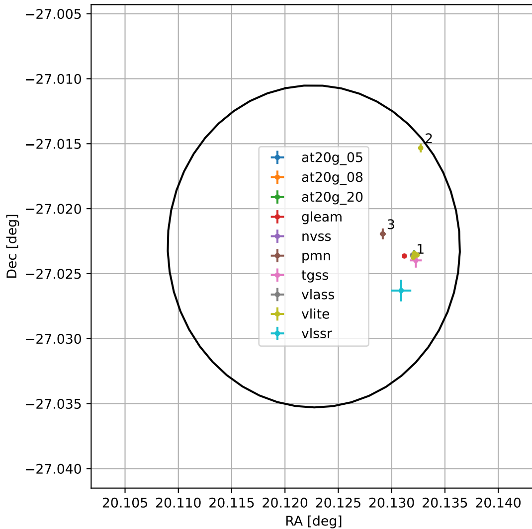
4FGL J0120.4-2701
