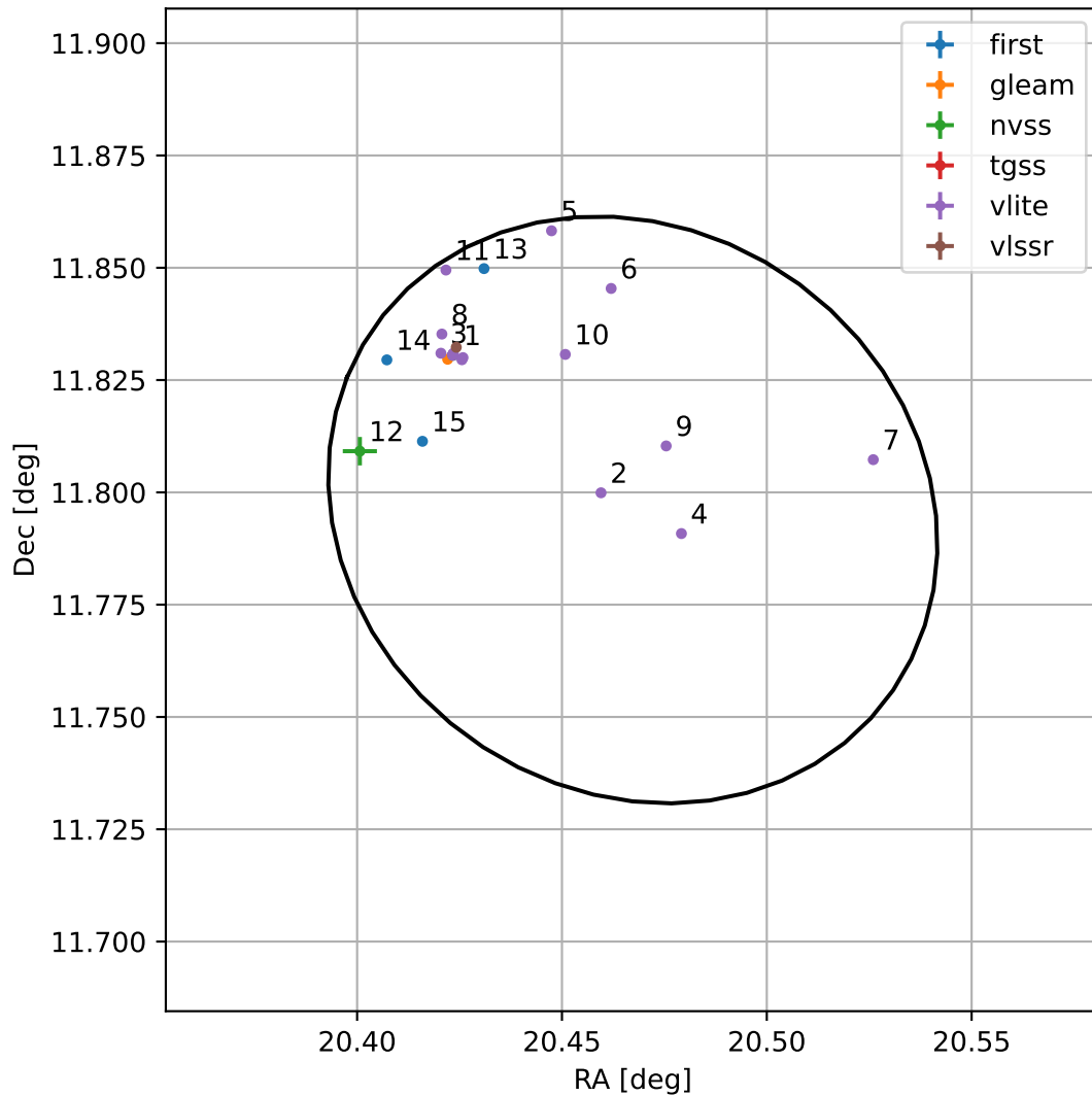
4FGL J0121.8+1147
