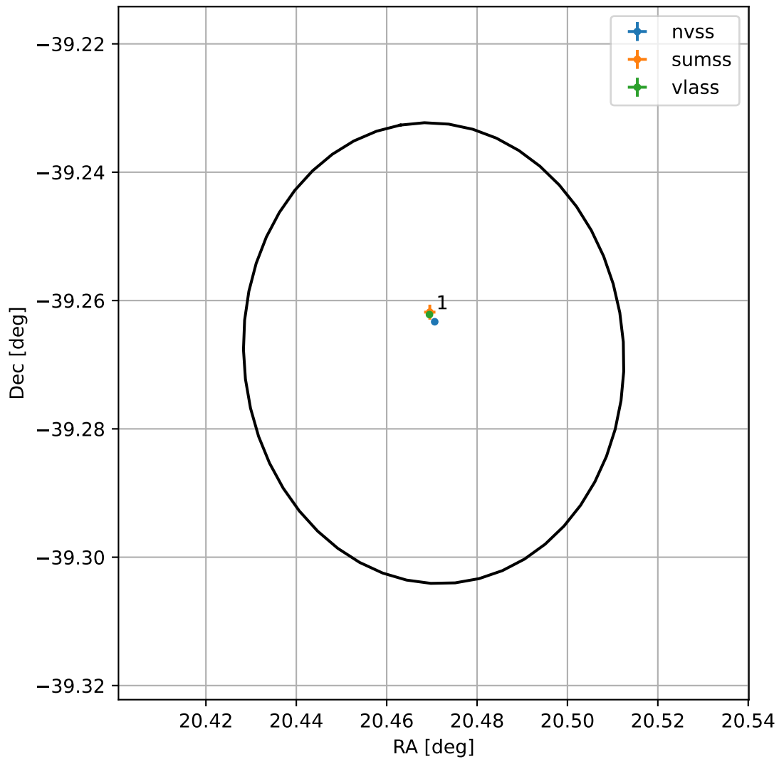
4FGL J0121.8-3916
