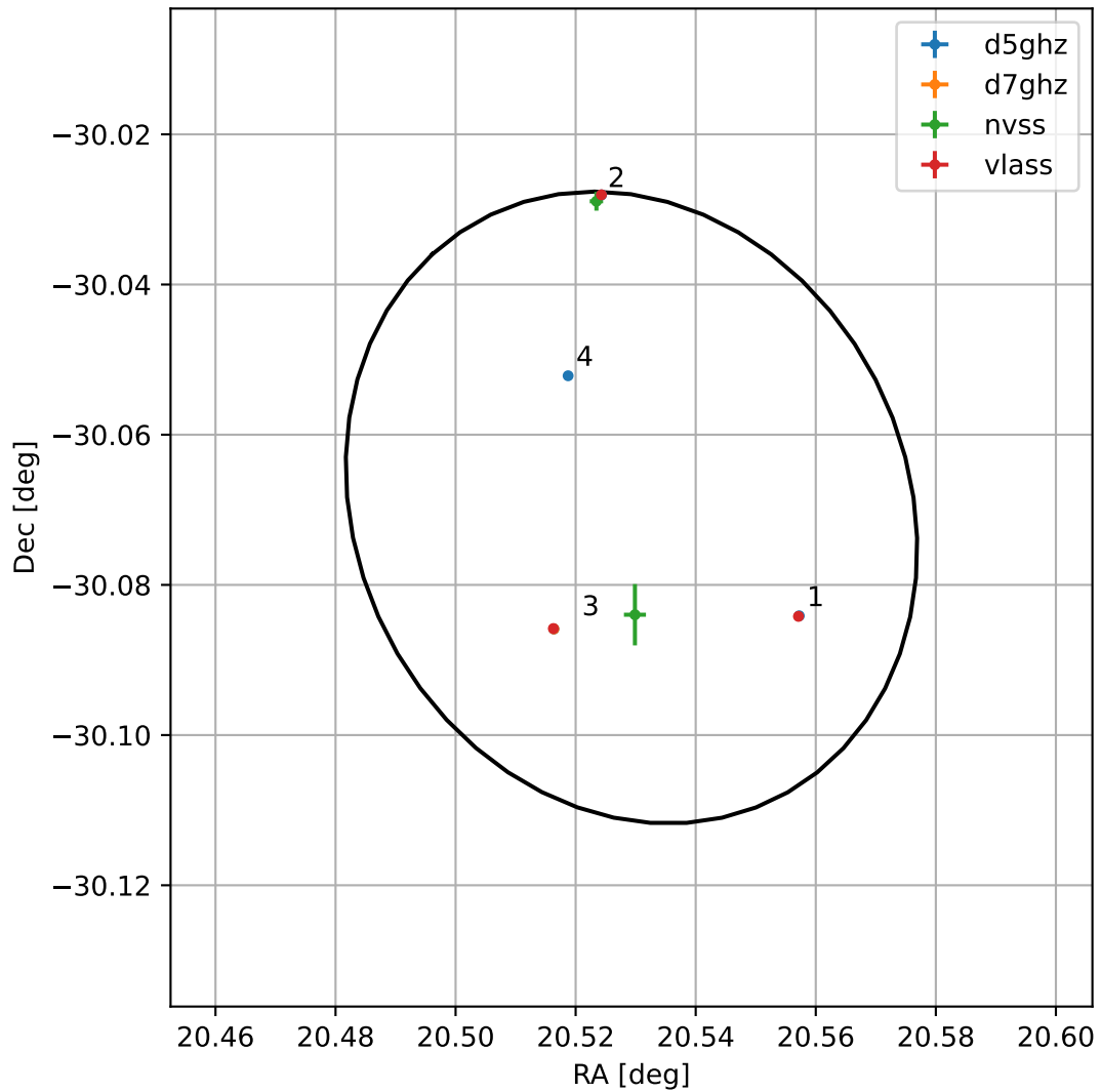
4FGL J0122.1-3004
