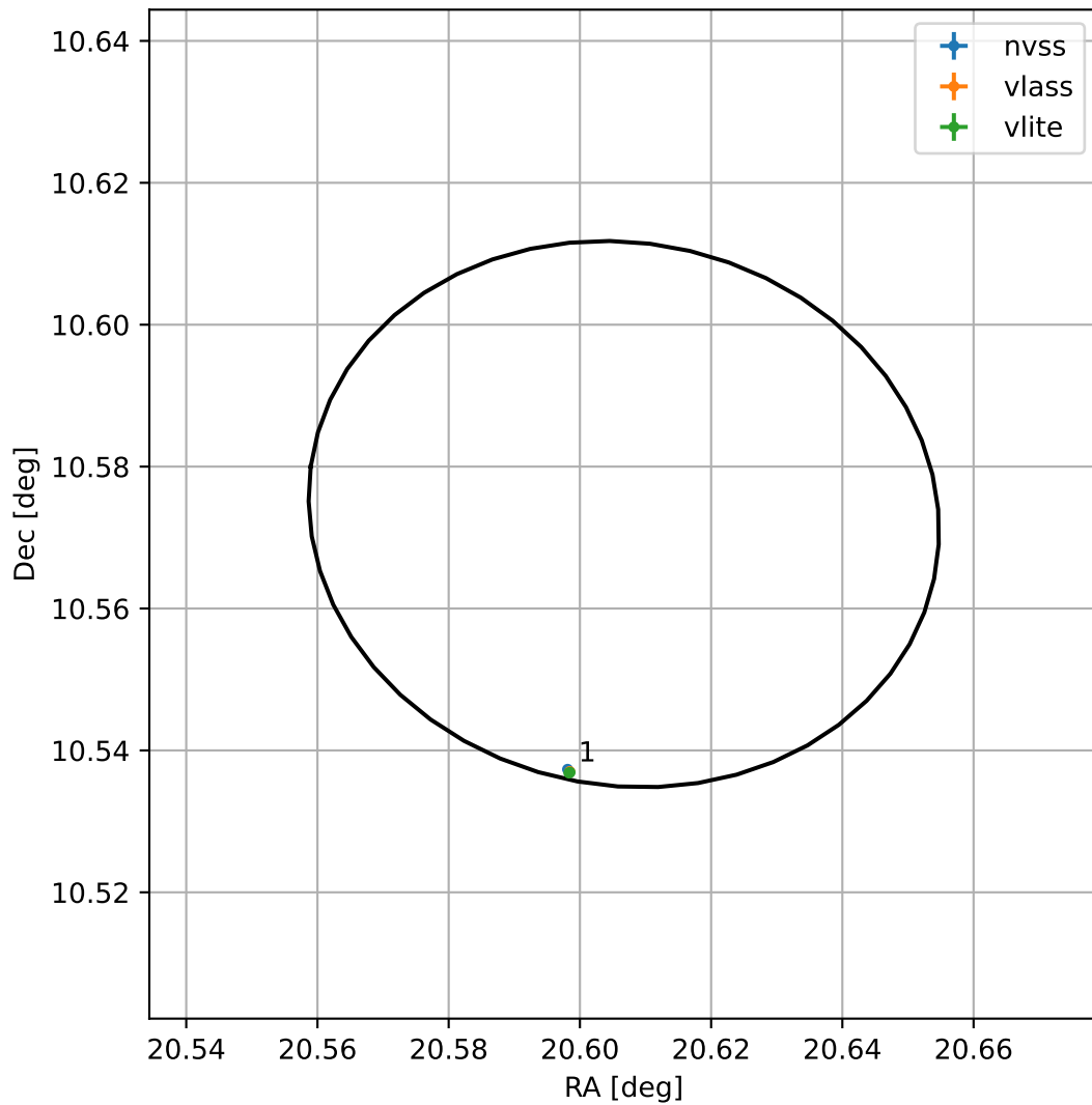
4FGL J0122.4+1034
