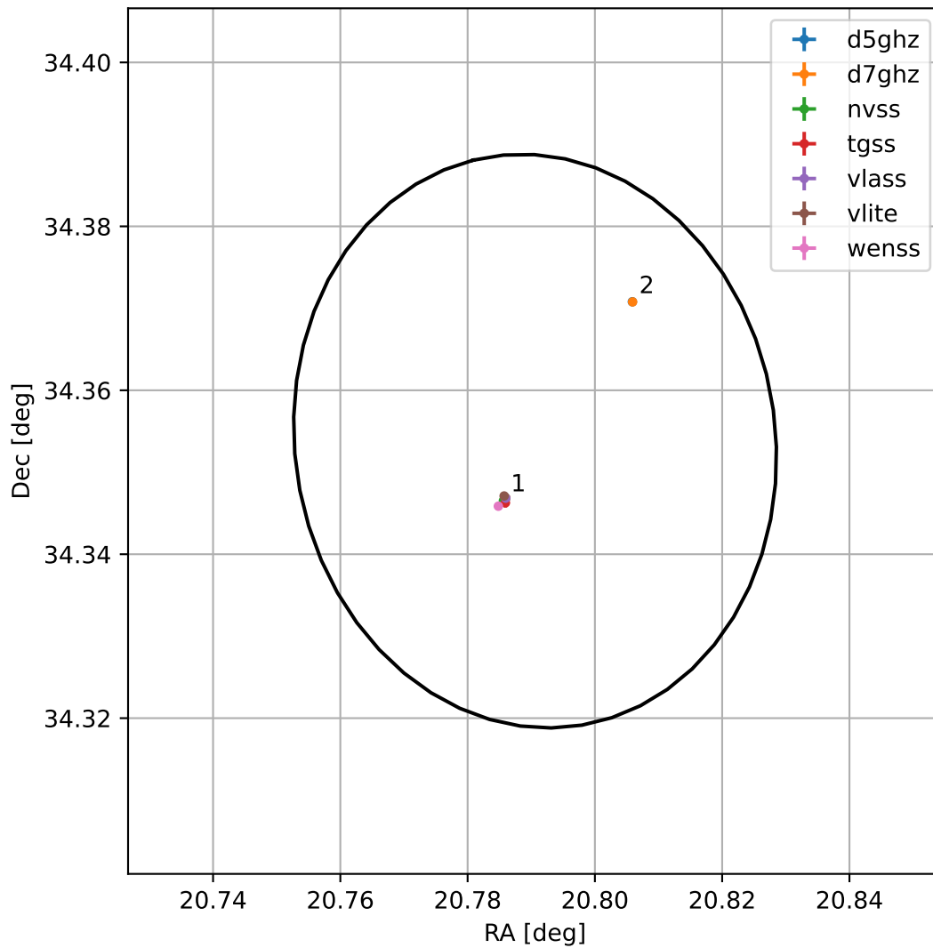
4FGL J0123.1+3421
