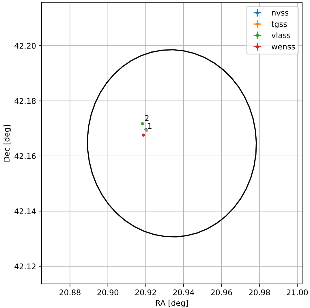
4FGL J0123.7+4209
