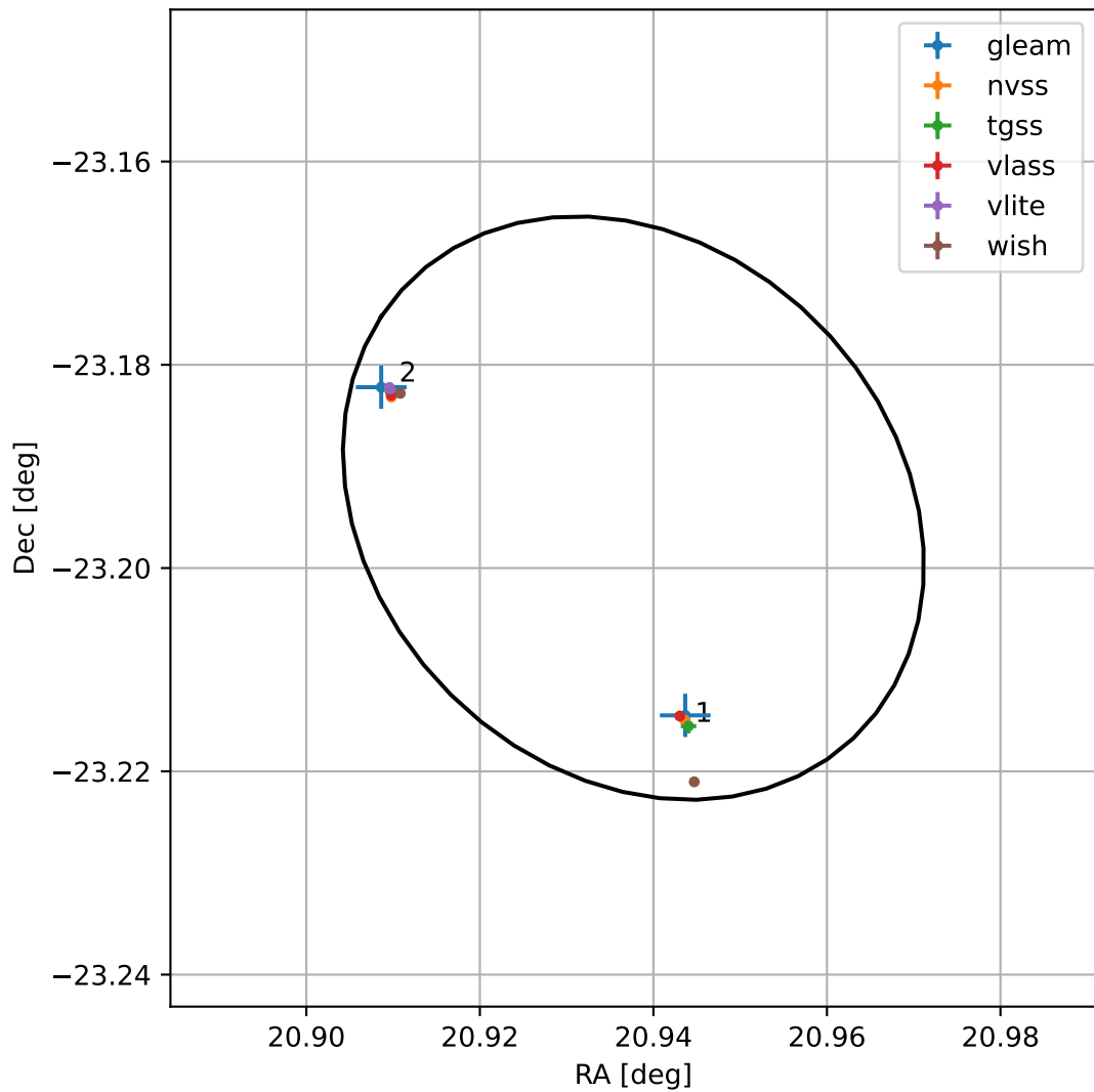
4FGL J0123.7-2311
