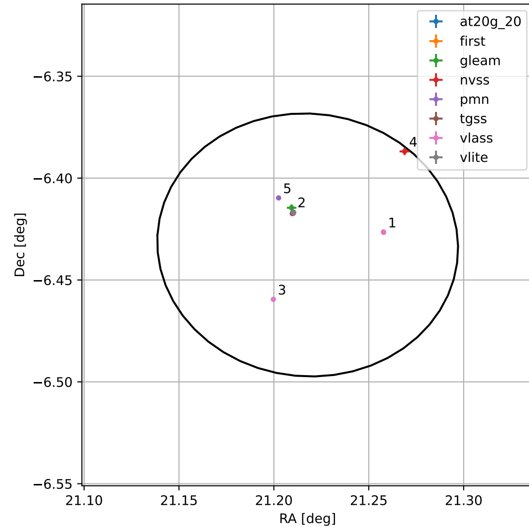
4FGL J0124.8-0625
