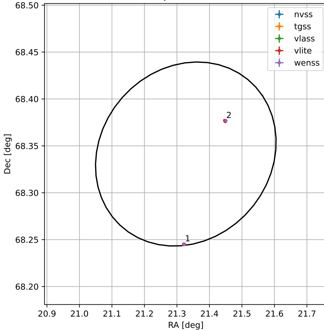
4FGL J0125.3+6820
