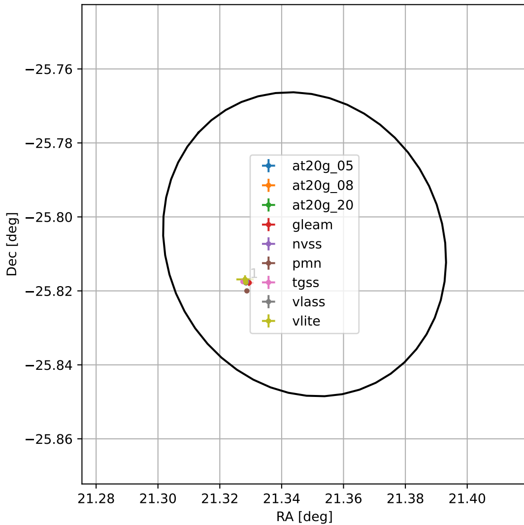
4FGL J0125.3-2548
