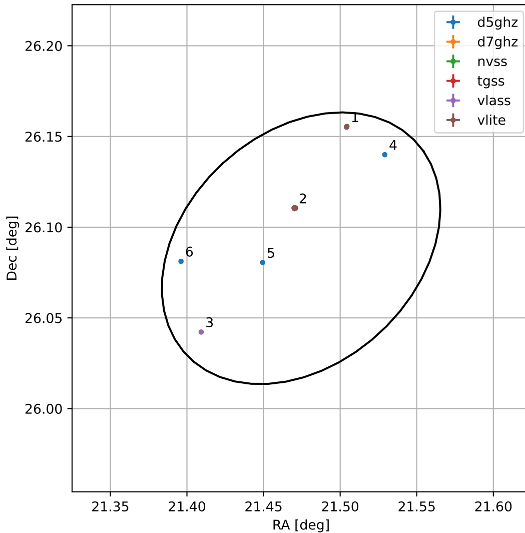
4FGL J0125.8+2605
