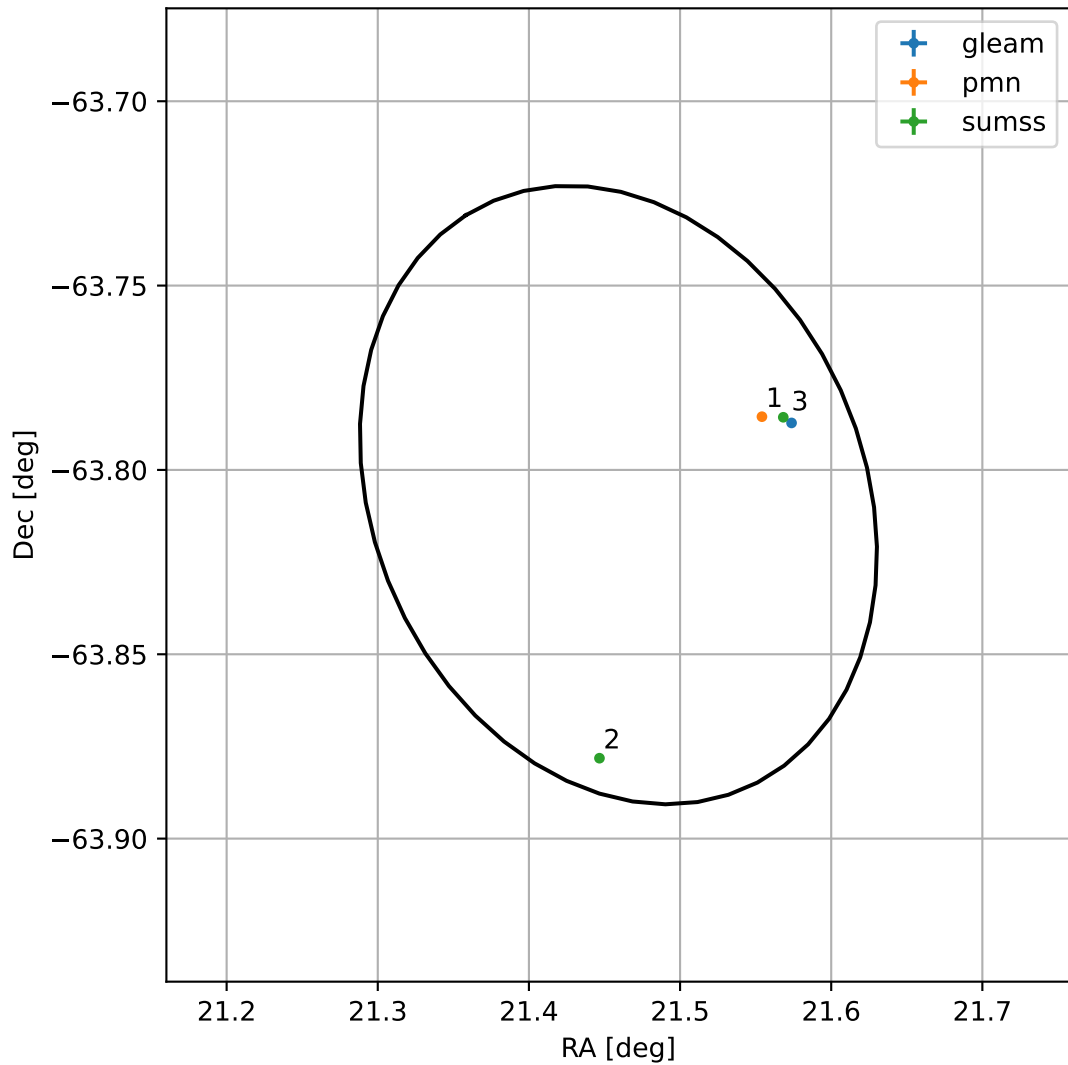
4FGL J0125.8-6348
