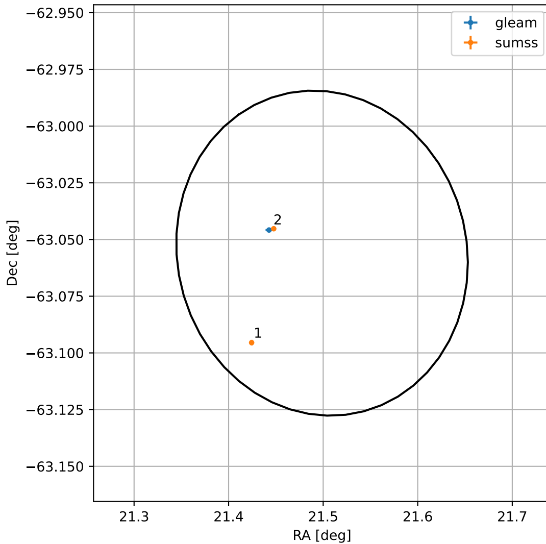
4FGL J0125.9-6303
