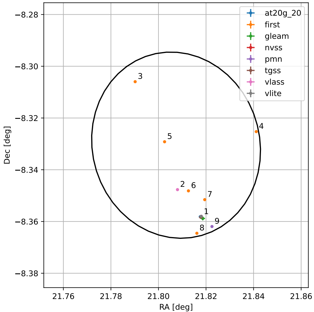
4FGL J0127.2-0819
