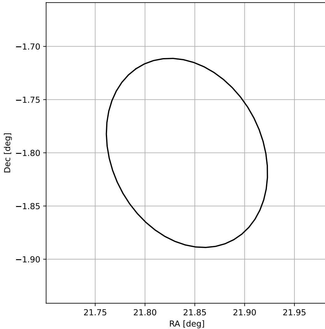
4FGL J0127.3-0148
