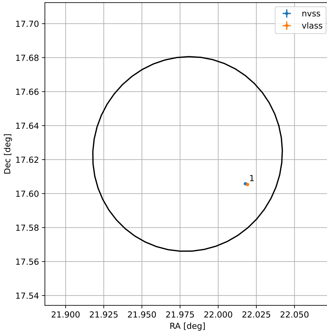
4FGL J0127.9+1737
