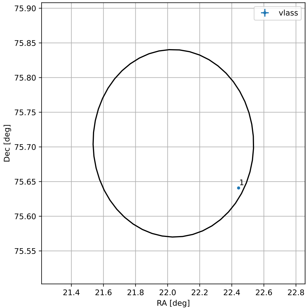
4FGL J0128.1+7542
