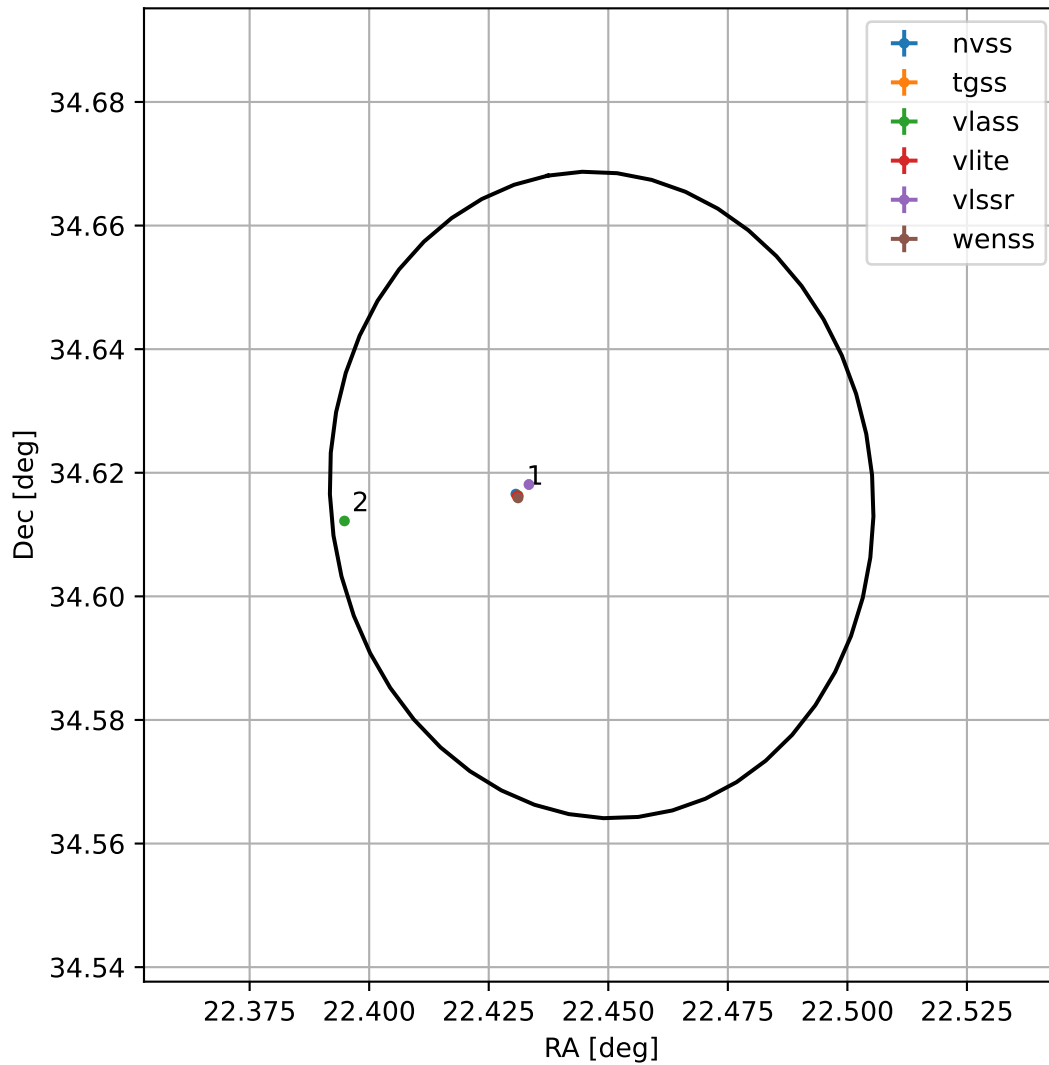
4FGL J0129.7+3436
