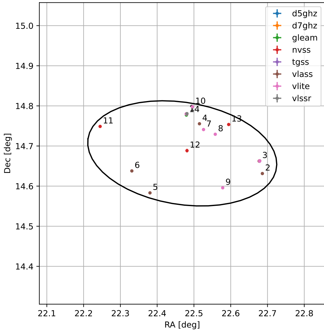
4FGL J0129.8+1440
