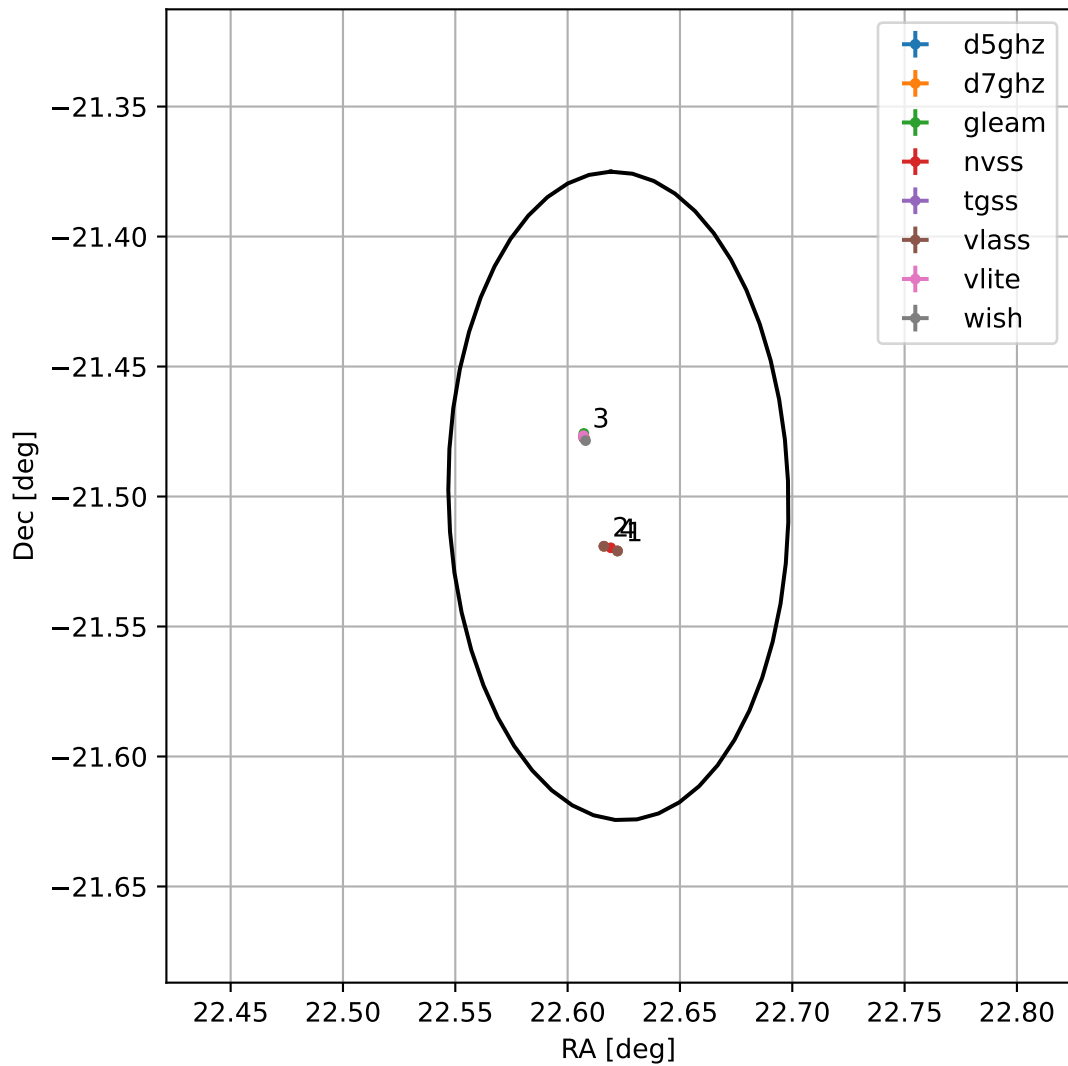
4FGL J0130.4-2129
