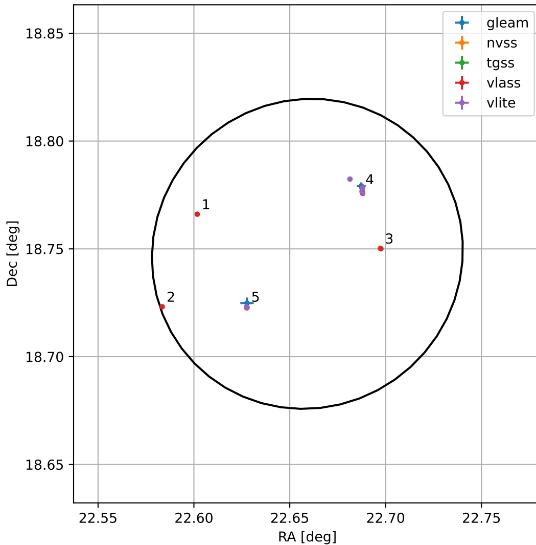
4FGL J0130.6+1844
