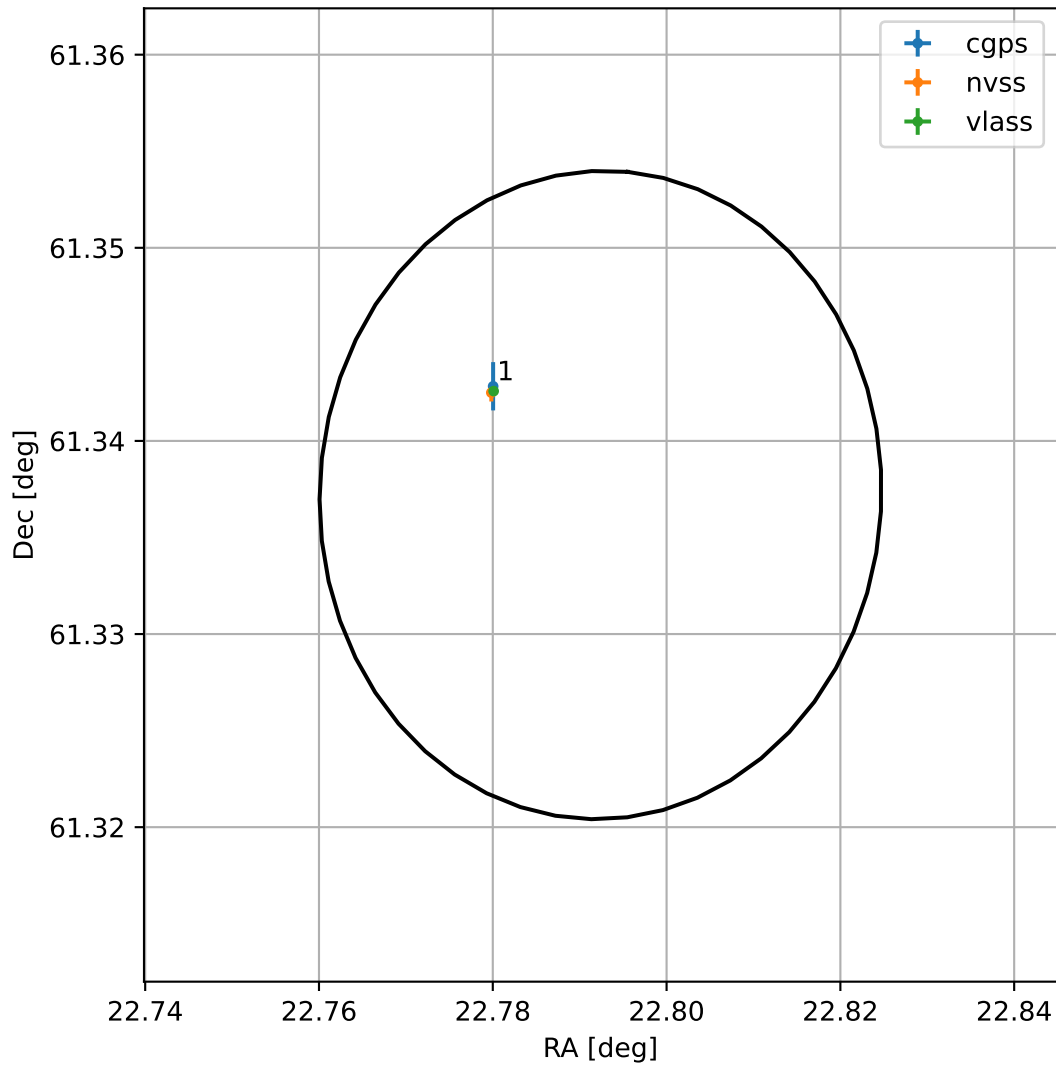
4FGL J0131.1+6120
