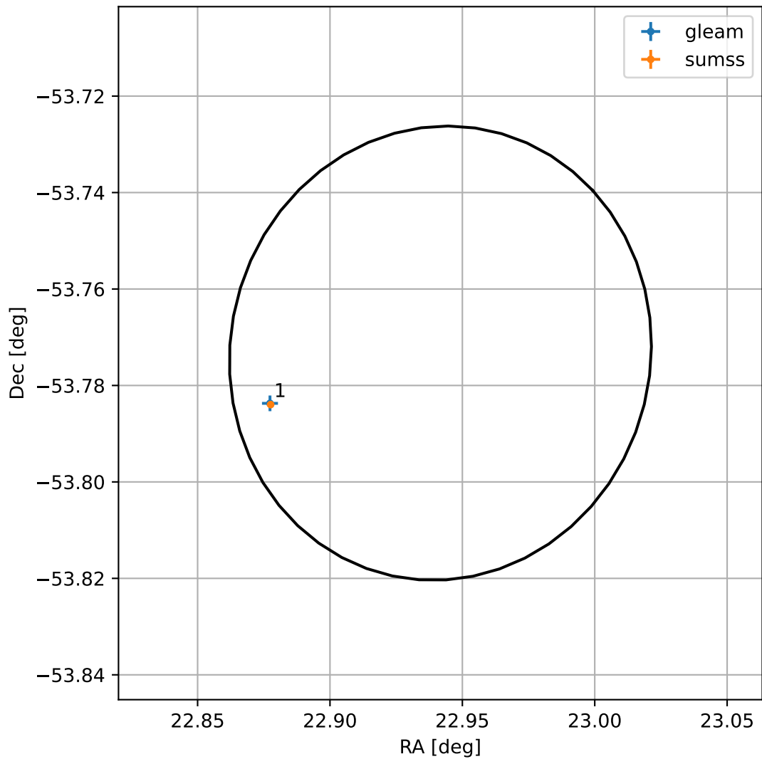
4FGL J0131.7-5346
