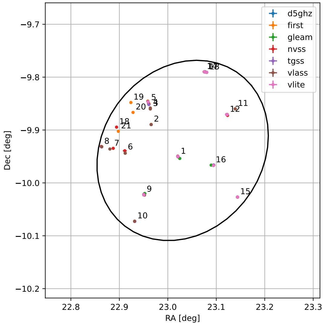
4FGL J0132.1-0956
