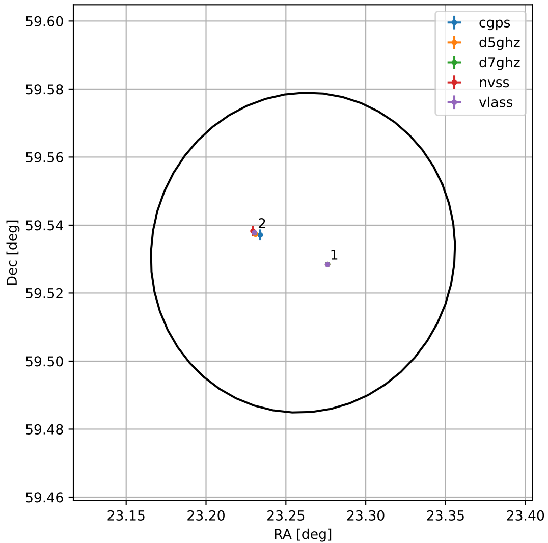
4FGL J0133.0+5931
