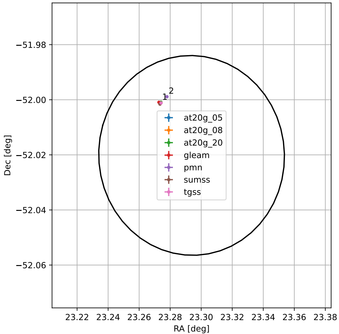
4FGL J0133.1-5201
