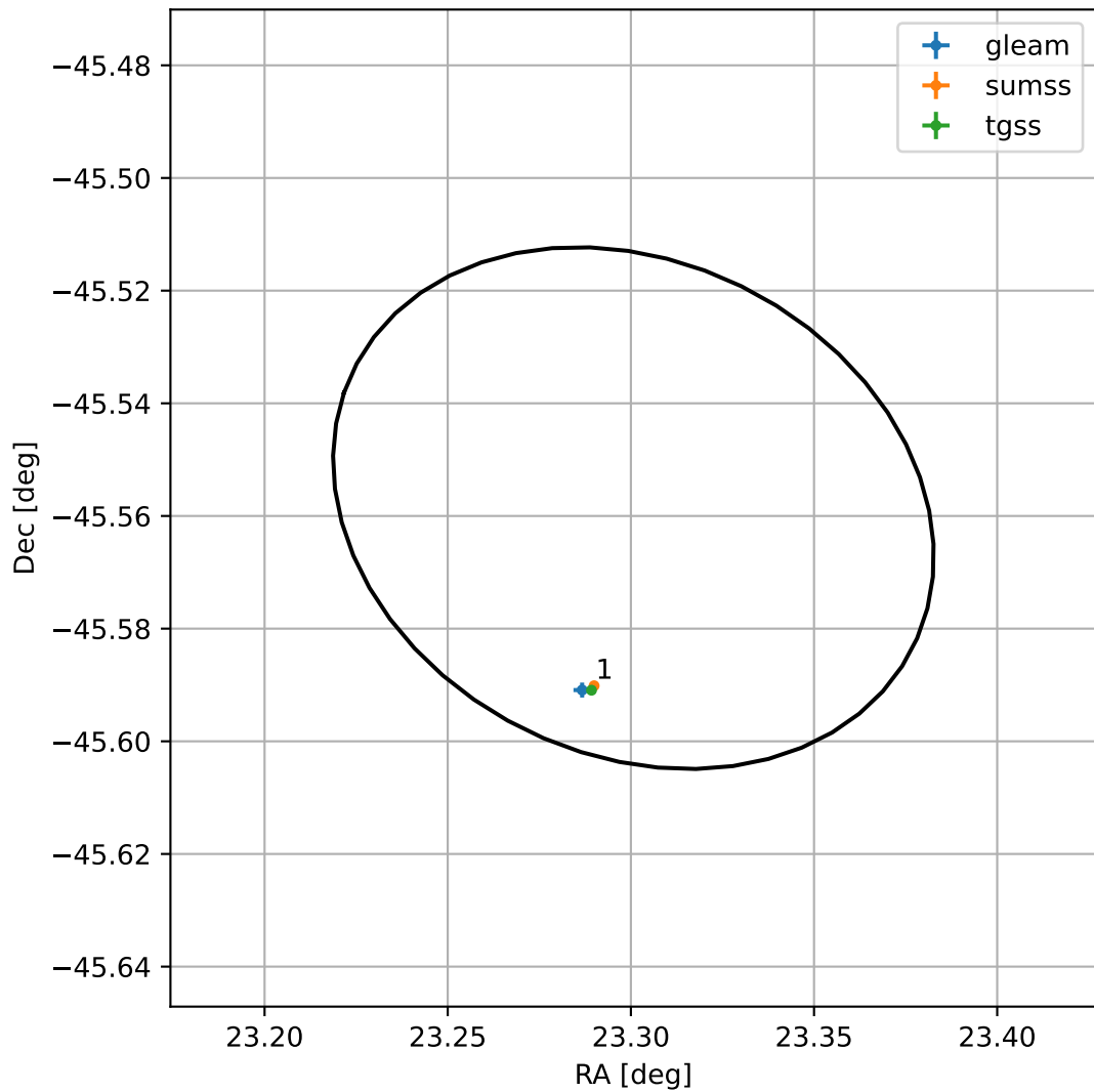
4FGL J0133.2-4533
