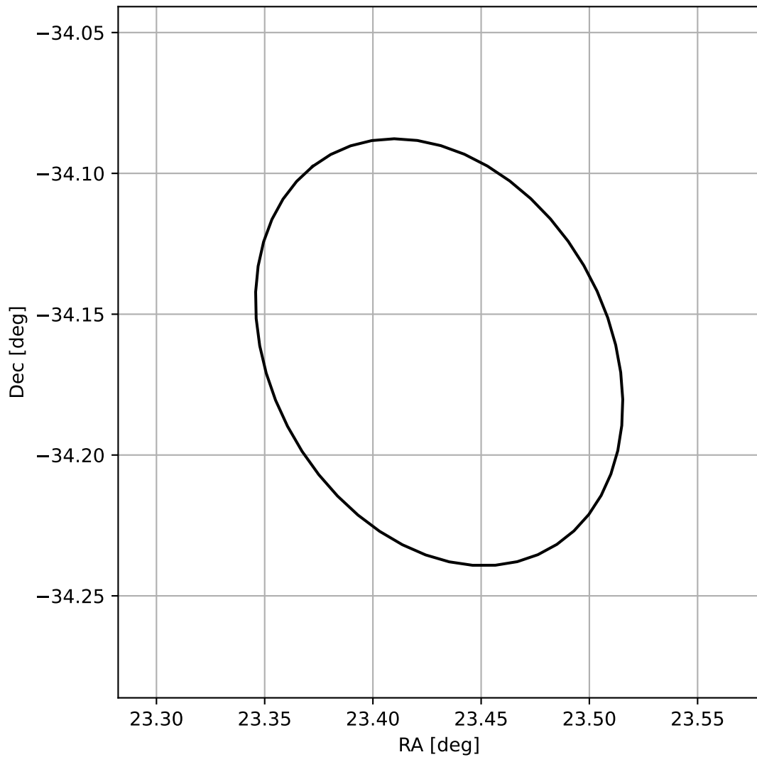
4FGL J0133.7-3409
