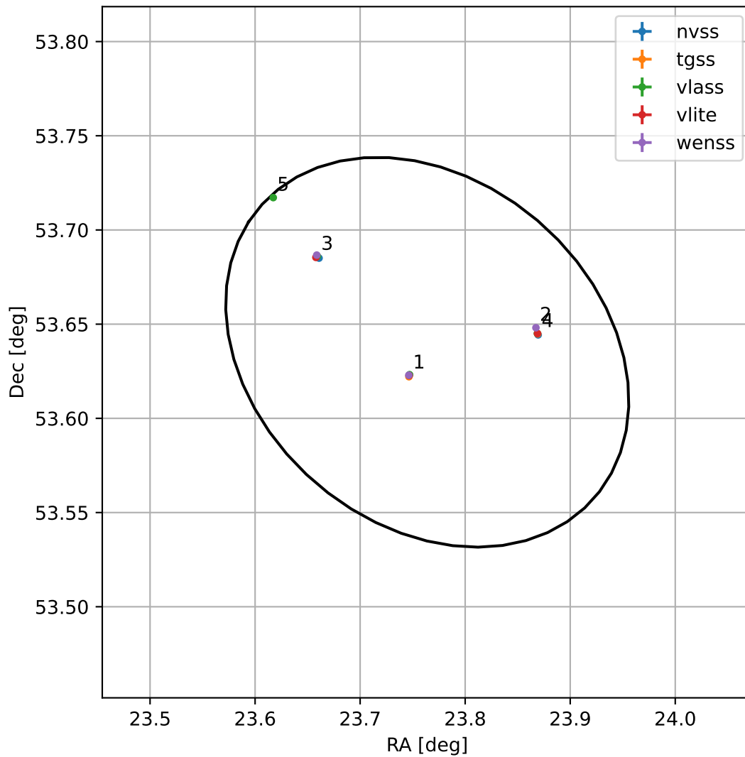
4FGL J0135.0+5338
