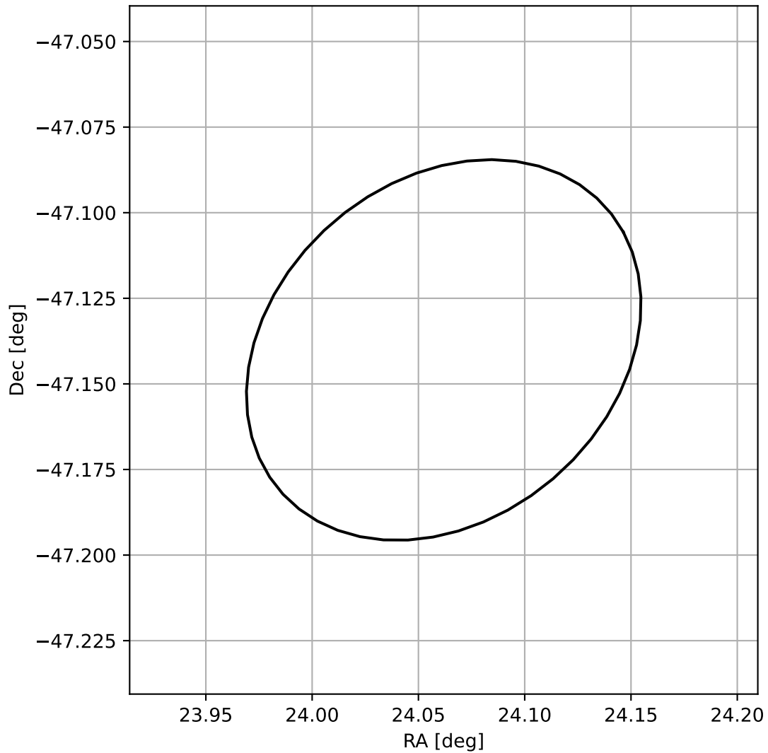
4FGL J0136.2-4708
