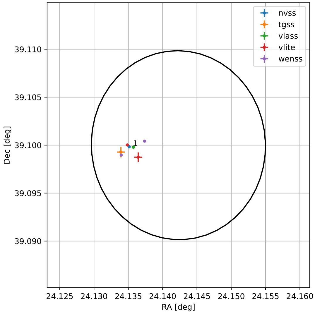
4FGL J0136.5+3906
