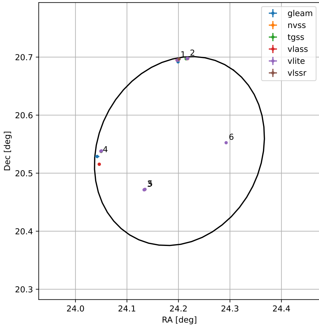
4FGL J0136.8+2032
